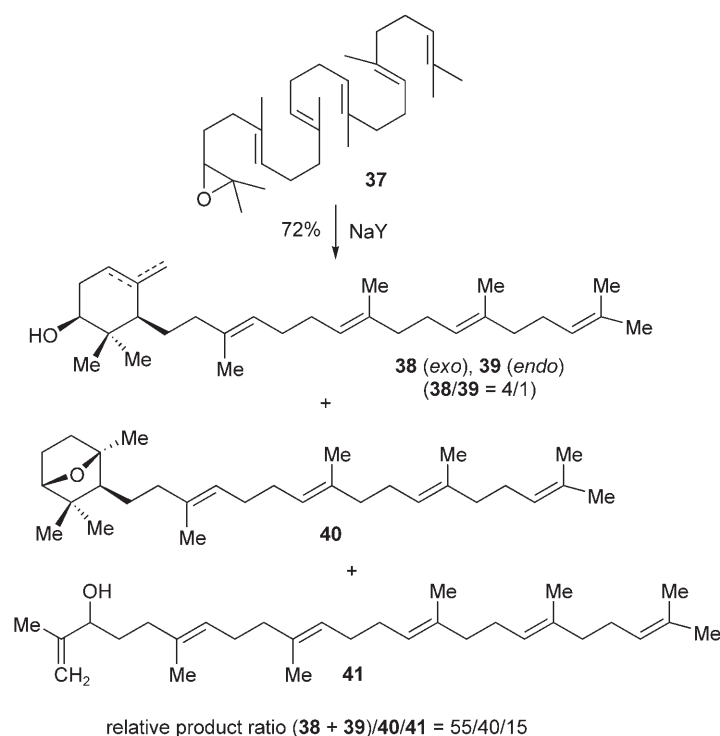
Scheme 5. Cyclization of 2,3-epoxysqualene ( 37 ) promoted by NaY.
