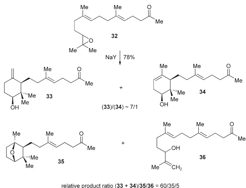
Scheme 4. NaY-promoted cyclization of epoxy trans,trans -farnesylacetone ( 32 ).
