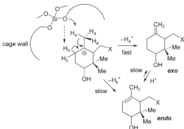
Scheme 7. Mechanistic arguments on the selective and regio-selective monocyclization of epoxy polyene terpenoids promoted by NaY.
