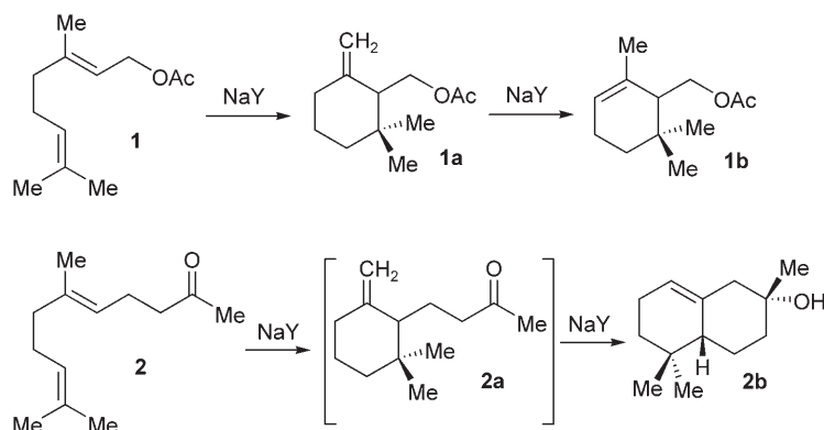
Scheme 1. Zeolite NaY-promoted cyclization of small terpenoids.
