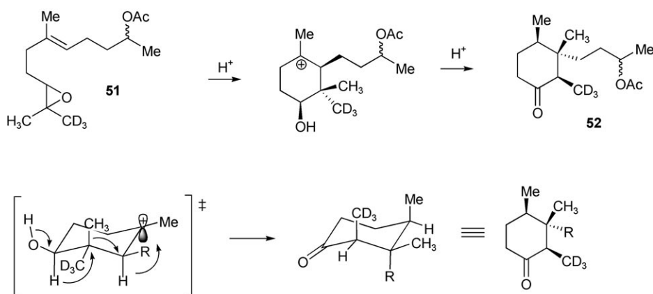
Scheme 11. Specific shift of the \text{CH}_3 relative to the \text{CD}_3 group during the formation of 52 .
