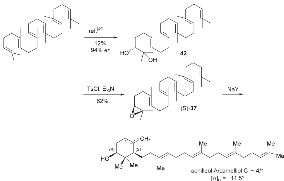
Scheme 6. Absolute configurations of (–)-achilleol A and (–)-camelliol C.
