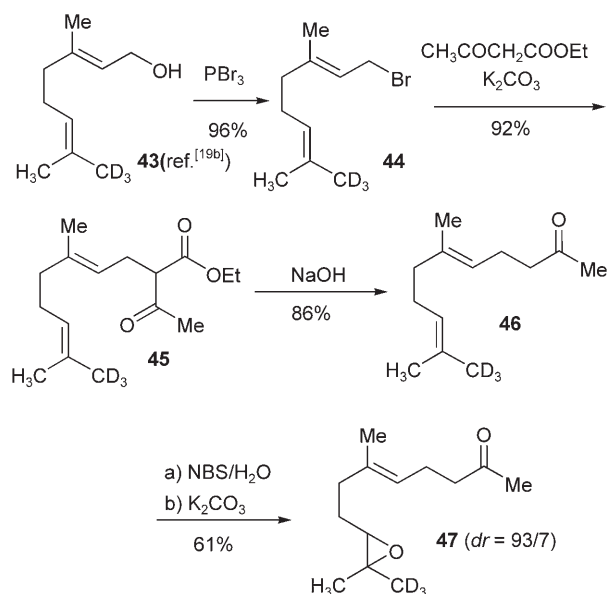
Scheme 8. Synthesis of the deuterium-labelled epoxy geranylacetone 47 .
