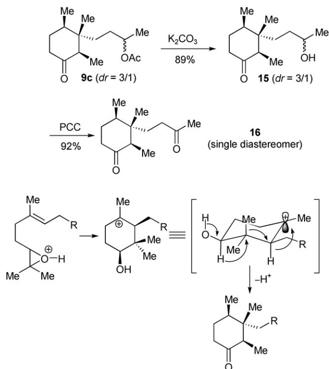
Scheme 2. Structural characterization of by-product 9c , and a plausible mechanism for its formation.
