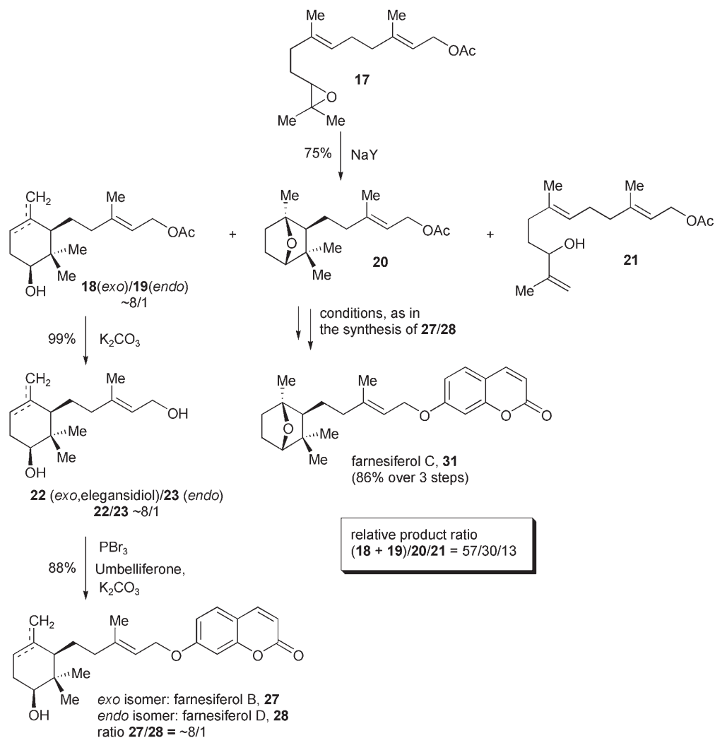
Scheme 3. Monocyclization of 10,11-epoxyfarnesyl acetate ( 17 ) promoted by NaY: synthesis of elegansidiol and farnesiferols B–D.
