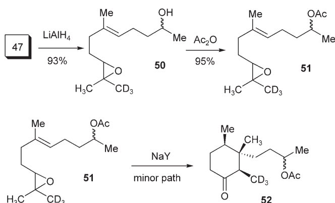
Scheme 10. Synthesis of the labeled epoxide 51 , and the stereochemistry of the by-product 52 isolated after treatment with \text{NaY} .
