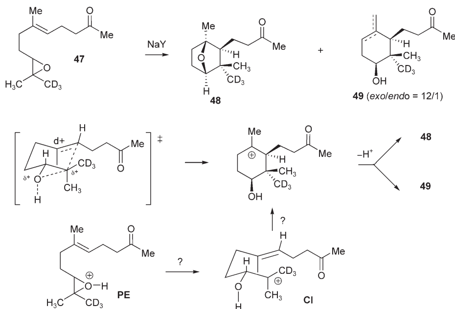
Scheme 9. Stereochemistry for the cyclization of 47 @NaY, and the proposed mechanism.
